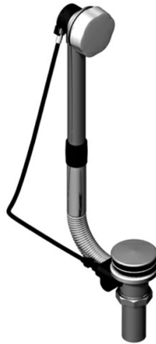
16" ADJUSTABLE CABLE DRIVEN TELESCOPIC WASTE & OVERFLOW (SOLID BRASS)
