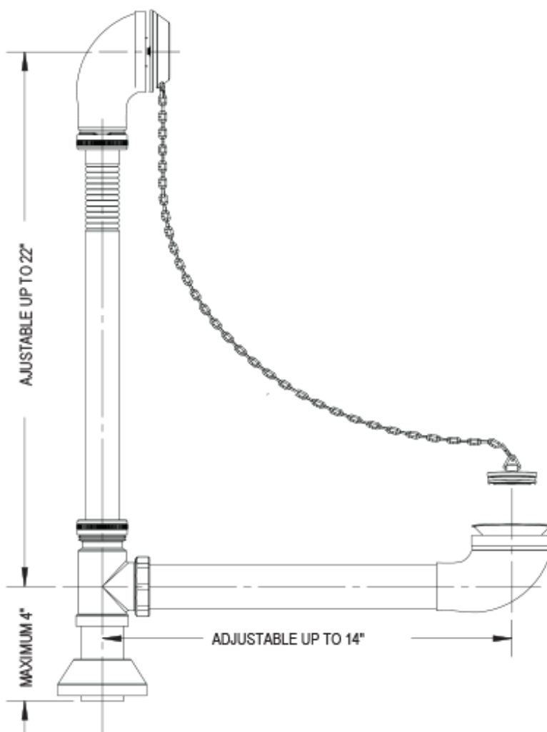
22" EXPOSED ADJUSTABLE PLUG & CHAIN TUBULAR WASTE & OVERFLOW (SOLID BRASS)
