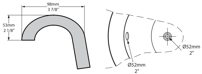
Rim detail
