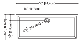
plan view
